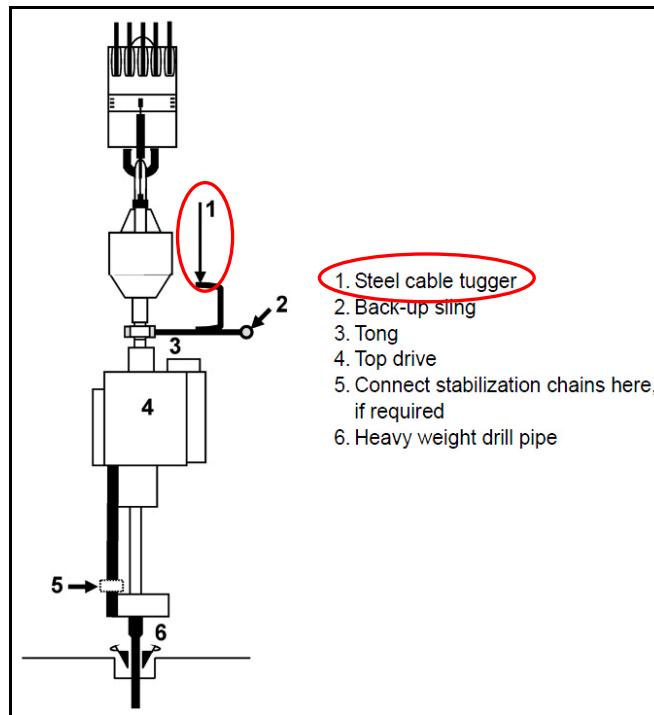
Figure 1: Using a steel cable tugger line in place of cat line tugger
